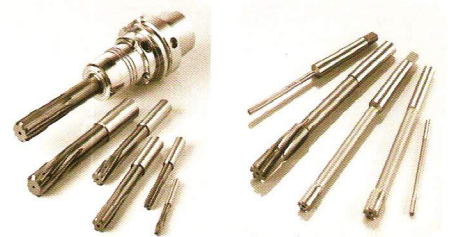
Reamer
