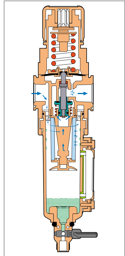
Figure 27. GENERAL PURPOSE FILTER/REGULATOR
