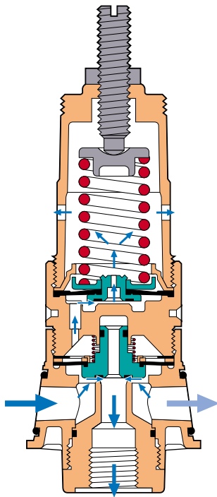
Figure 32. INTERNAL PILOT RELIEF VALVE
