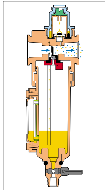
Figure 29. OIL-FOG LUBRICATOR
