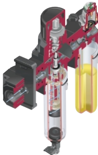
Figure 35. EXCELON SYSTEM
