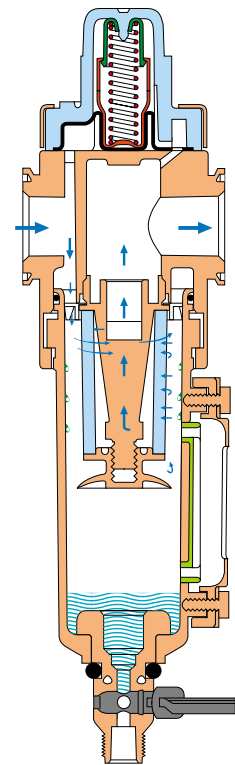
Figure 13. GENERAL PURPOSE FILTER
