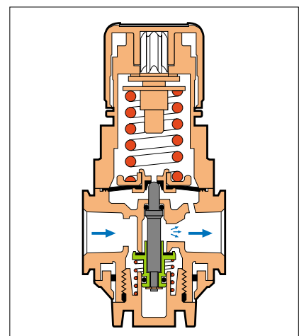
Figure 22. GENERAL PURPOSE REGULATOR
