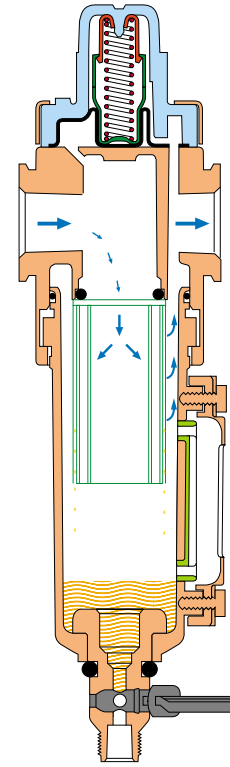
Figure 14. 'PURAIRE' COALESCING FILTER
