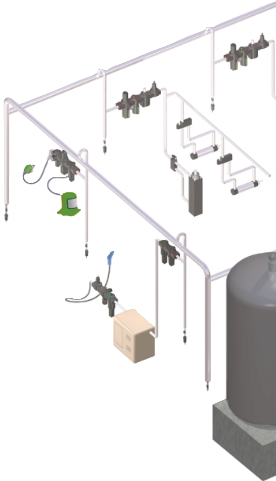
Figure 1. Compressed air installation, showing examples of air preparation applications. See details on pages 4 and 5.
