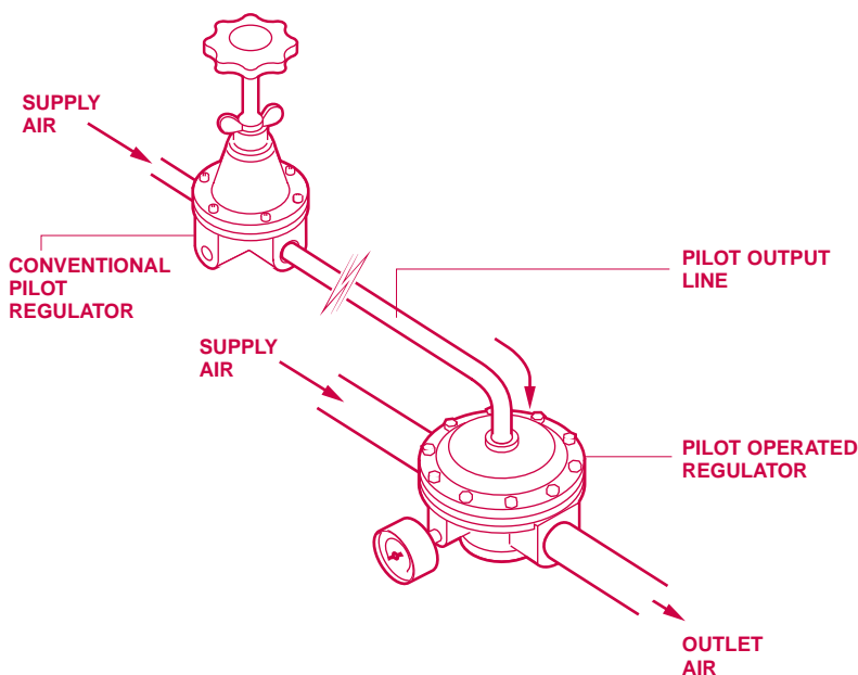
Figure 23. A TYPICAL PILOT OPERATED REGULATOR INSTALLATION.
