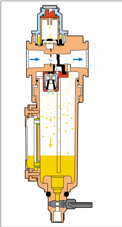
Figure 30. MICRO-FOG LUBRICATOR
