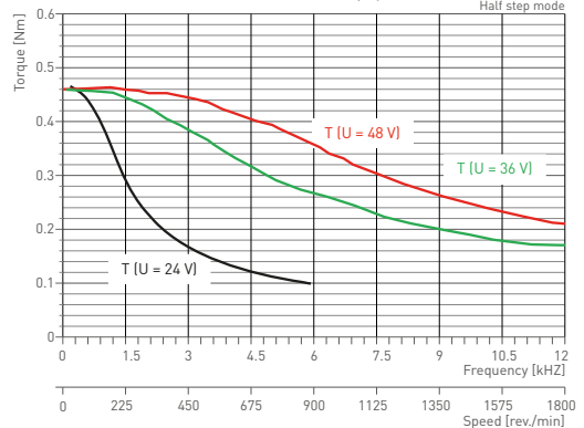
phyBASIC 56-3 / NEMA 23 Half step mode
