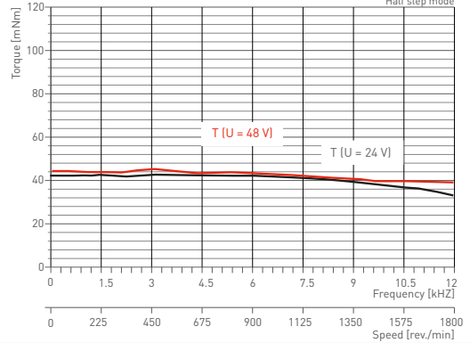
phyBASIC 42-3 / NEMA 17 Half step mode
