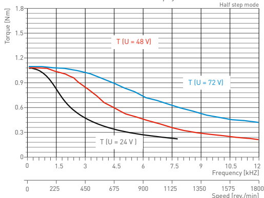
phyBASIC 86-1 / NEMA 34 Half step mode
