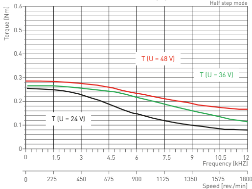
phyBASIC 56-2 / NEMA 23 Half step mode
