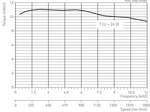
phyBASIC 42-1 / NEMA 17 Half step mode
