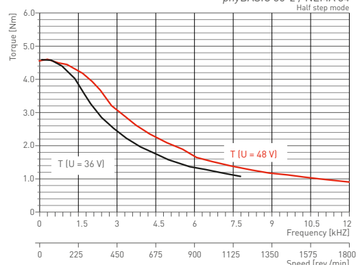
phyBASIC 86-2 / NEMA 34 Half step mode
