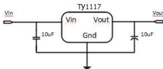
Application circuit of Ty1117 fixed version
