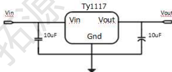
Application circuit of Ty1117 fixed version
