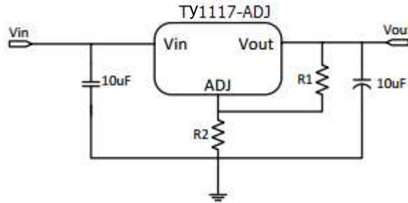
Application Circuit of Ty1117 -ADJ
