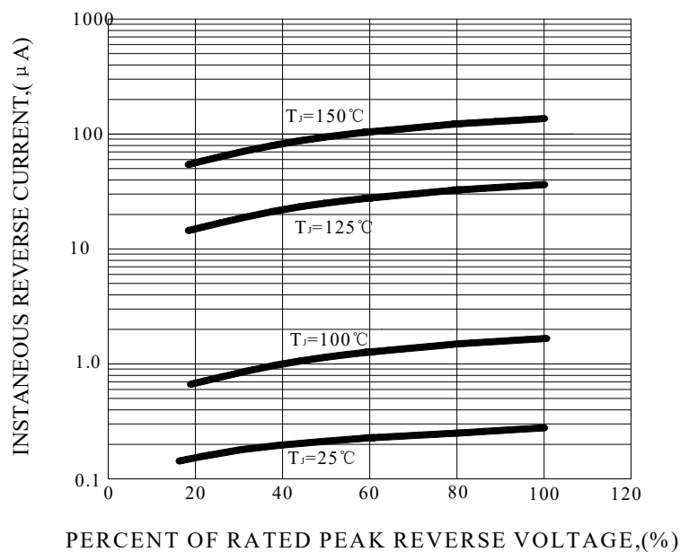
FIG.5-TYPICAL REVERSE CHARACTERISTICS
