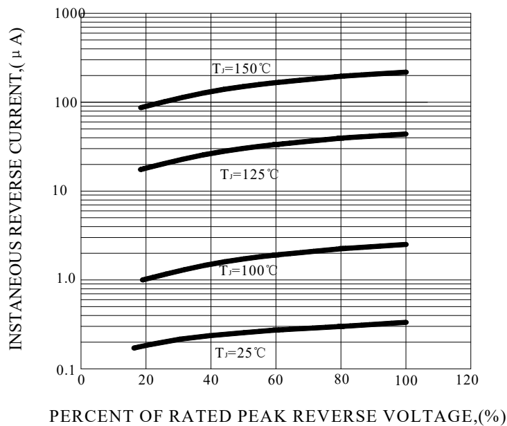
FIG.5-TYPICAL REVERSE CHARACTERISTICS
