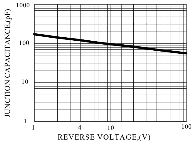
FIG.4-TYPICAL JUNCTION CAPAOTANCE
