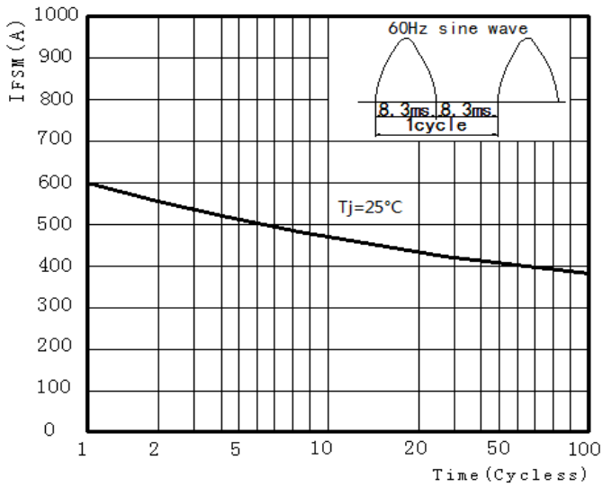
FIGURE 3. Peak Surge Forward Capability
