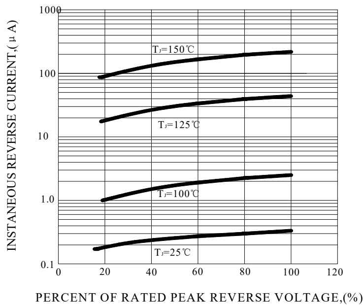
FIG.5-TYPICAL REVERSE CHARACTERISTICS
