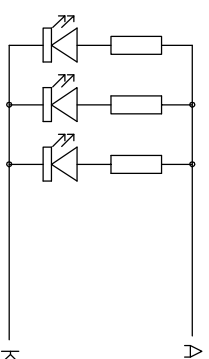
Backlight Circuit Scale=free
